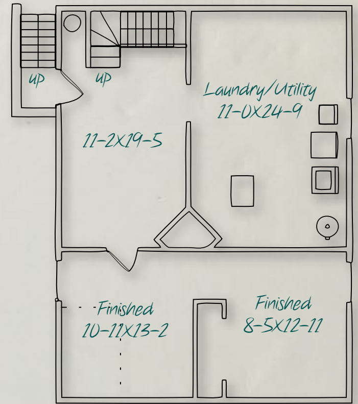
Main House Lower Floor
