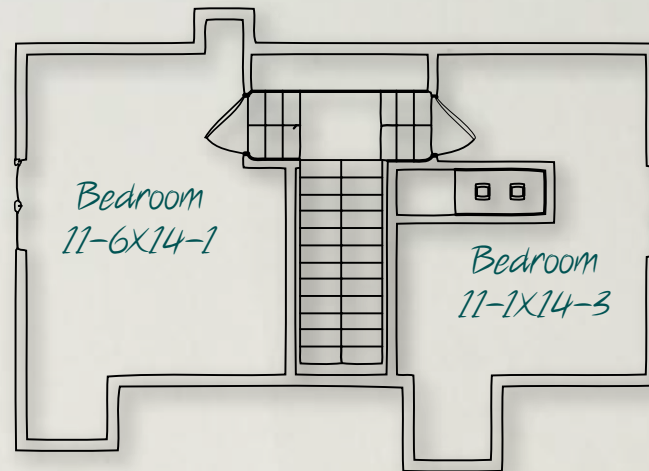
Cottage Upper Floor
